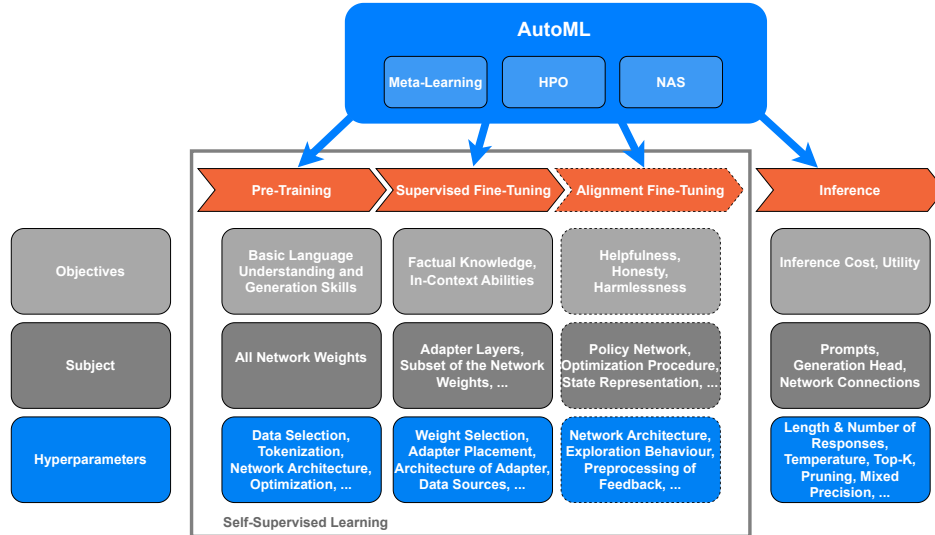
Figure 1: AutoML can be used in all stages of the LLM lifecycle and needs to be adjusted to the different objectives, hyperparameters, and design decisions of each stage. The graphic depicts exemplary objectives, subjects of optimization, and associated hyperparameters. Due to computational constraints, the stages are considered separately, one after the other. Alignment is a non-mandatory stage.
