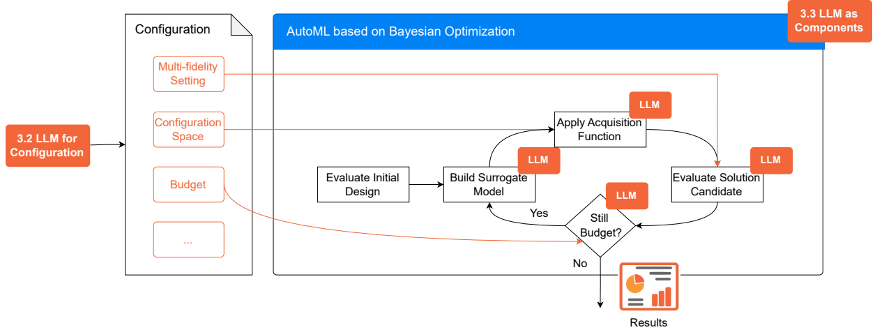
Figure 3: Visualization of the potential of LLMs for the configuration of AutoML (Section 3.2) and LLMs as components of AutoML systems (Section 3.3) at the example of a AutoML process based on Bayesian Optimization.
